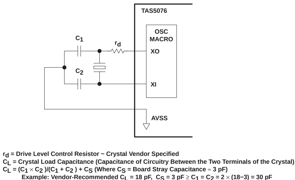
Figure 2–1. Crystal Circuit
